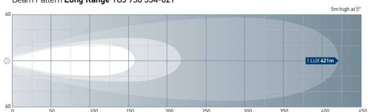
Beam Pattern Long Range 1GJ 958 334-021
