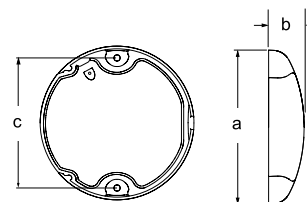
Dimensions a = 129.5mm / 5.10" b = 29.5mm / 1.16" c = 110mm / 4.33"
